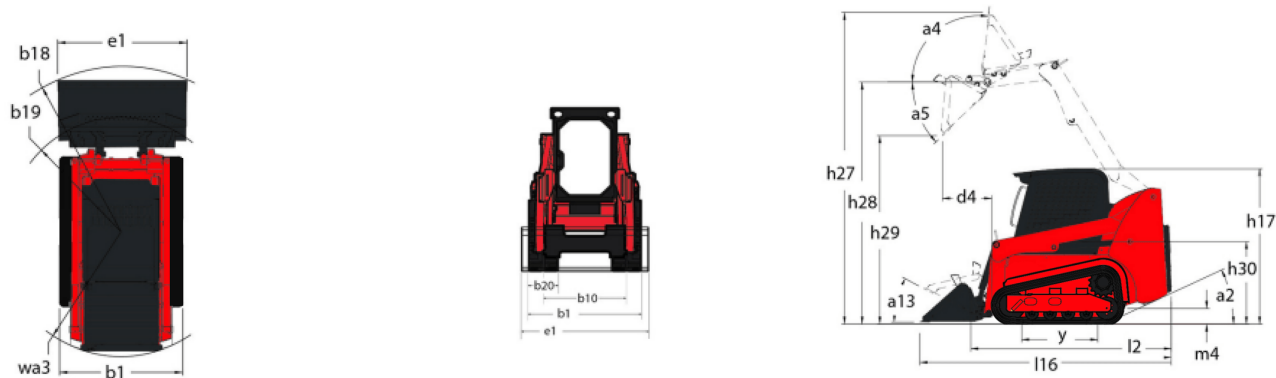
2100VT - Dimensional drawing
